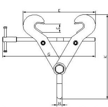
Fixed Jaw
