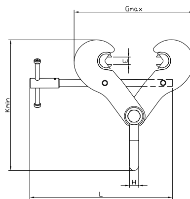
Swivel Jaw
